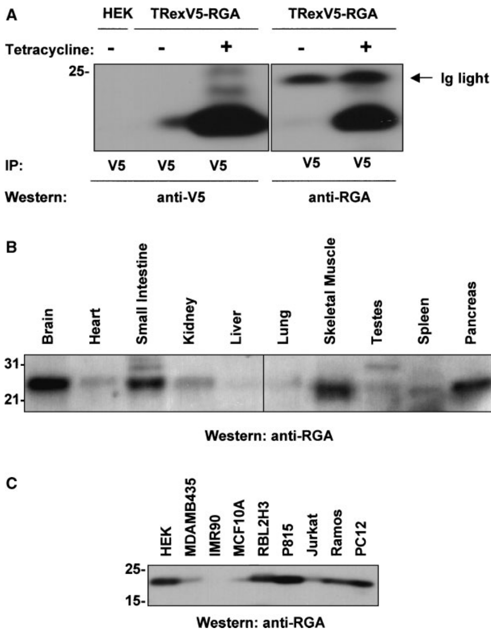
Fig. 2. A: Novel anti-recombinase gene activator (RGA) antibody recognizes RGA protein in an over-expression system. TRexRGA cells, with V5-RGA expression under the control of a tetracycline-sensitive transcriptional repressor, were constructed. TRexRGA were exposed to vehicle or 1 \mu g/ml tetracycline for 16 h at 37°C, to induce expression of V5-RGA. Triton X-100 lysates from 1 \times 10^7 TRexRGA cells were immunoprecipitated with 2 \mu g anti-V5. Immunocomplexes were resolved by 10% SDS-PAGE and electrotransferred. V5-RGA was visualized by Western blotting in 0.5 \mu g/ml anti-V5 antibody ( left panel ) or 1 \mu g/ml anti-RGA ( right panel ). Second lane of left-hand panel displays some signal carry-over. B: Novel anti-RGA antibody recognizes a 24 kDa protein in various human tissues. A
